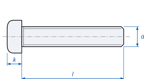
Thread Rolling Screw DIN 7500 - dimensions
