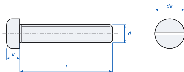
Seating Screw DIN 15237 - dimensions
