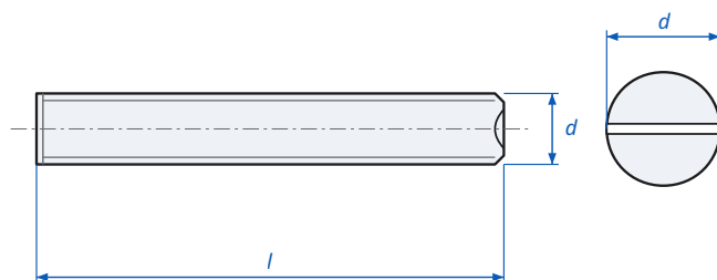
Slotted Headless Screw with Chamfered End DIN 427 - dimensions
