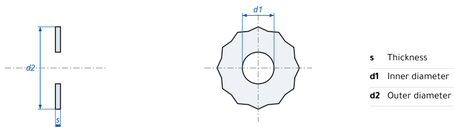
Internal Serrated Lock Washer DIN 6798J - dimensions
