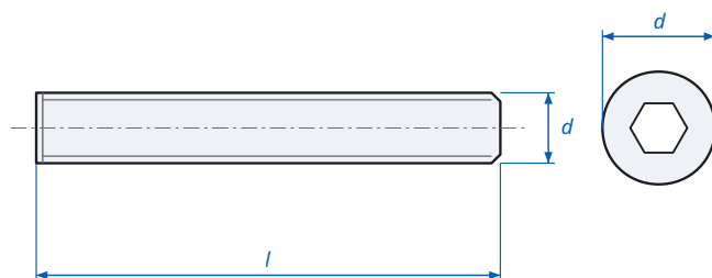
Hex Socket Set Screw Flat Point DIN 913 / ISO 4026 - dimensions
