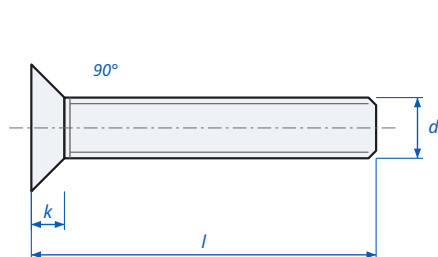
Slotted Countersunk Head Screw DIN 963 / ISO 2009 - dimensions
