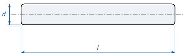
Parallel Pin Hardened DIN 6325 / ISO 8734 - dimensions
