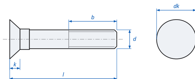
Flat Countersunk Square Neck Bolt DIN 605 - dimensions
