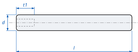
Pull Dowel Pin (Holo-Krome) - dimensions
