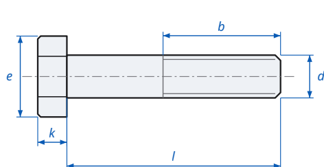
Hex Fit Bolt for Steel Structures DIN 7968 - dimensions
