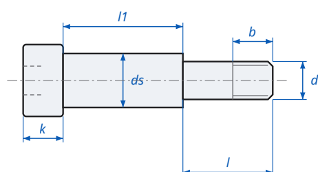
Socket Shoulder Screw ASME B18.3 - dimensions
