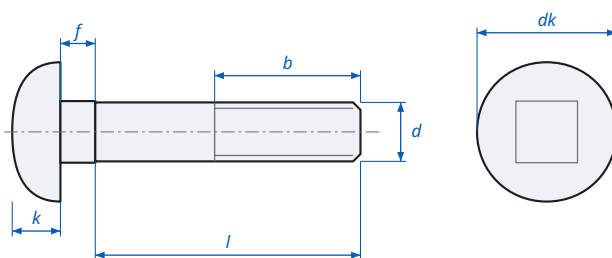
Mushroom Head Square Neck Bolt (Carriage Bolt) DIN 603 - dimensions
