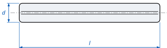
Slotted Spring Pin ANSI B18.8.2 - dimensions
