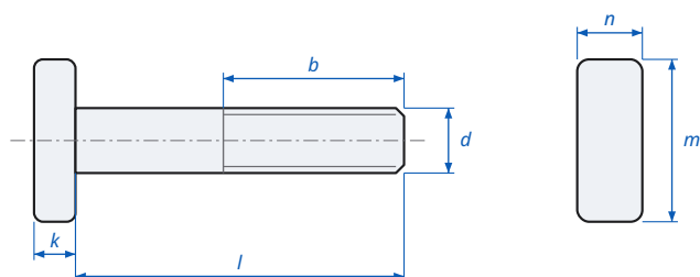
T-Head Bolt with Square Neck DIN 186 - dimensions
