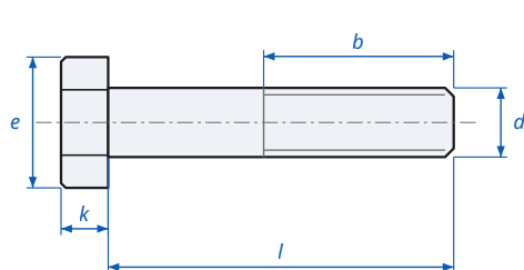
Hex Head Bolt Fine Thread DIN 960 / ISO 8765 - dimensions
