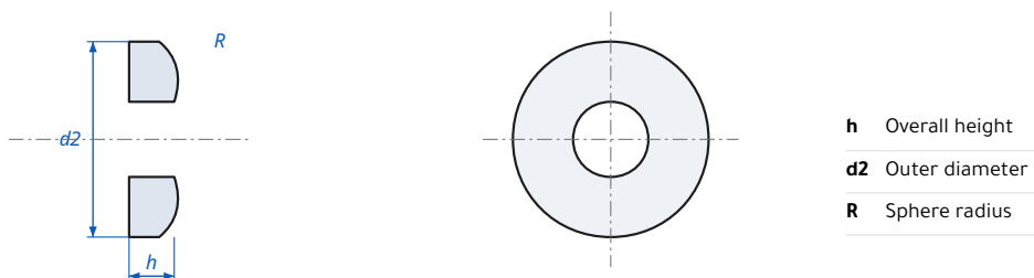
Conical Seat Washer DIN 6319D - dimensions
