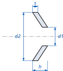
Conical Spring Washer DIN 6796 - dimensions
