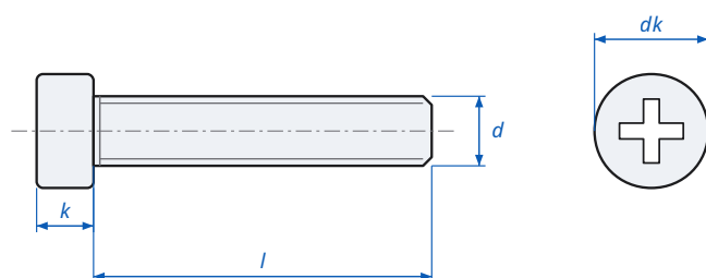
Cross Recessed Raised Cheese Head Screw DIN 7985 / ISO 7045 - dimensions
