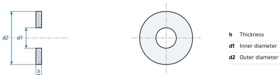
Thick Flat Washer DIN 7349 - dimensions
