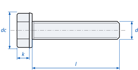
Hex Head Screw Plug with Collar DIN 910 - dimensions
