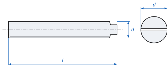
Slotted Set Screw Long Dog Point DIN 417 - dimensions
