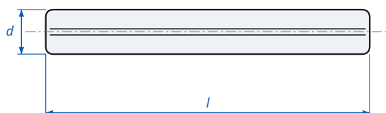
Slotted Spring Pin Heavy Duty DIN 1481 / ISO 8752 - dimensions
