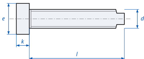
Square Head Bolt with Short Dog Point DIN 479 - dimensions
