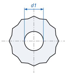
External Serrated Lock Washer DIN 6798A - dimensions
