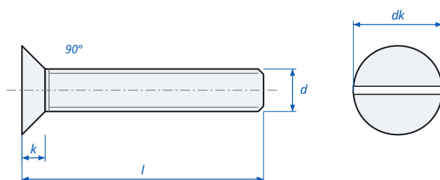
Slotted Countersunk Head Screw DIN 963 / ISO 2009 - dimensions
