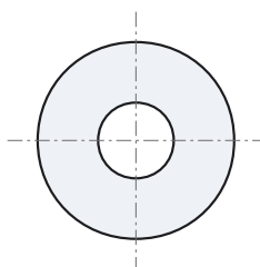
Flat Washer Chamfered DIN 125B / ISO 7090 - dimensions
