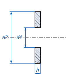
Flat Washer Chamfered DIN 125B / ISO 7090 - dimensions
