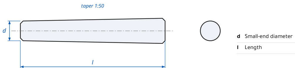
Taper Pin Form B DIN 1B / ISO 2339 - dimensions
