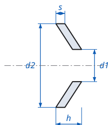
Conical Knurled Spring Washer NFE 25-511 - dimensions
