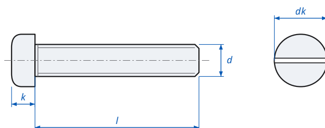
Slotted Pan Head Screw Large Head DIN 921 - dimensions
