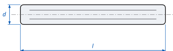
Grooved Pin Full-Length Parallel DIN 1473 - dimensions
