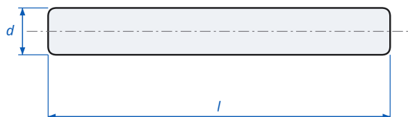
Hardened Dowel Pin ASME B18.8.5M - dimensions
