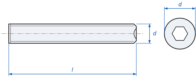
Hex Socket Set Screw Cup Point DIN 916 / ISO 4029 - dimensions
