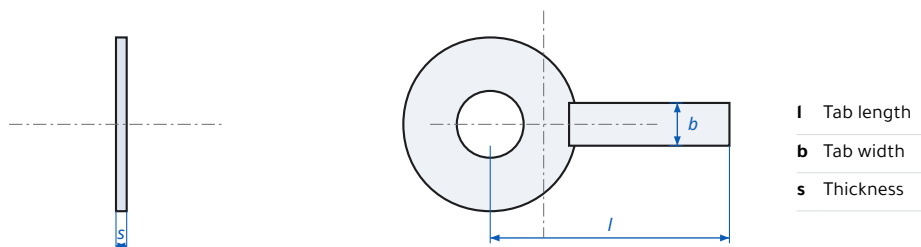
Tab Washer with External Tab DIN 432 - dimensions
