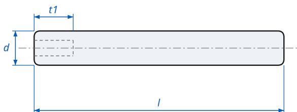
Taper Pin with Internal Thread DIN 7978A - dimensions
