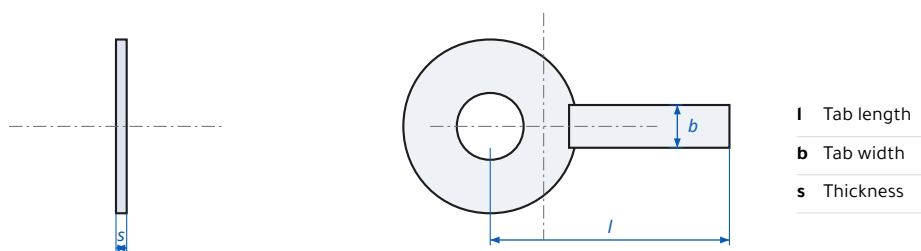
Tab Washer with Two Tabs DIN 463 - dimensions
