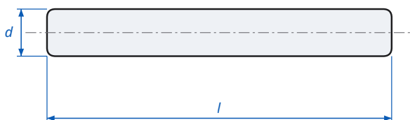
Coiled Spring Pin DIN 7343 / ISO 8750 - dimensions
