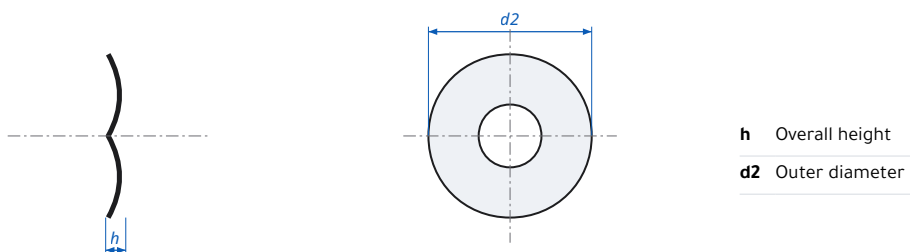
Curved Spring Washer DIN 137A - dimensions
