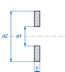
Flat Washer Large Series DIN 9021 - dimensions
