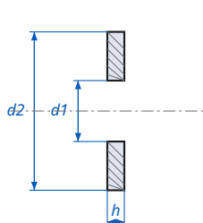
Flat Washer for Clevis Pins DIN 1440 - dimensions
