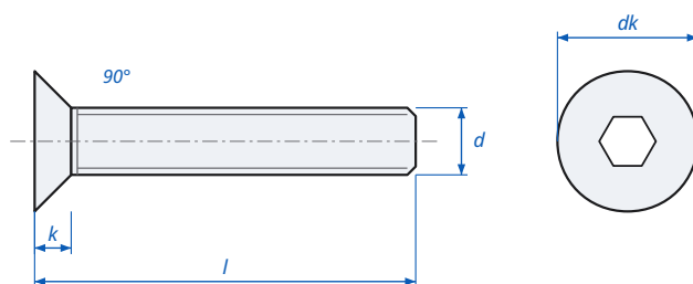
Flat Head Socket Cap Screw ASME B18.3 - dimensions
