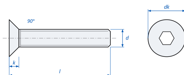
Hex Socket Countersunk Head Screw DIN 7991 / ISO 10642 - dimensions
