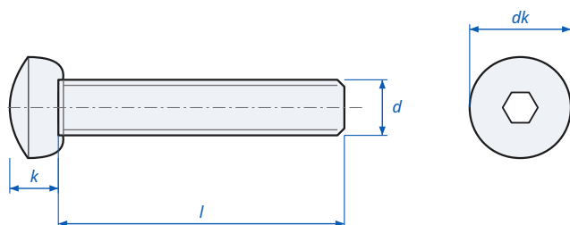
Button Head Socket Cap Screw ASME F912 - dimensions
