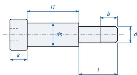
Hex Socket Shoulder Screw ISO 7379 - dimensions
