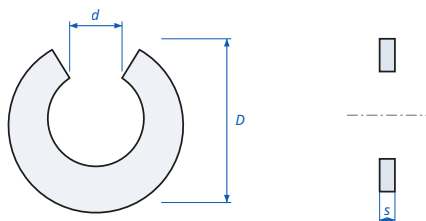
Retaining Washer for Shafts (E-Clip) DIN 6799 - dimensions
