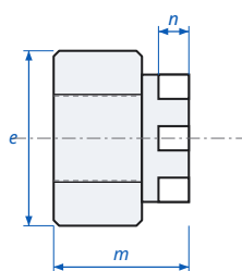
Hex Thin Castle Nut DIN 979 - dimensions
