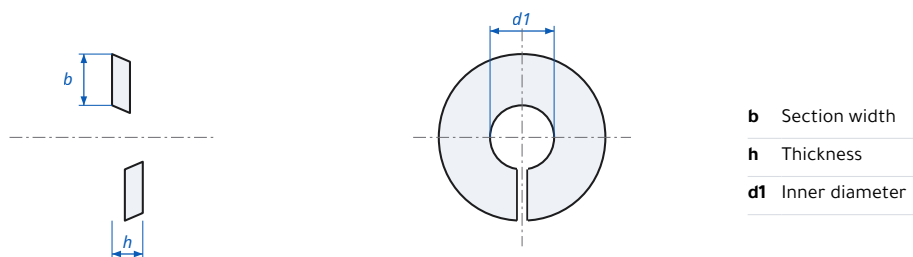
Curved Spring Washer Form A DIN 128A - dimensions
