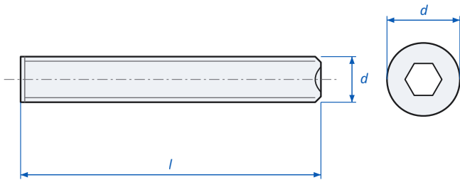
Jam Screw (Holo-Krome) - dimensions
