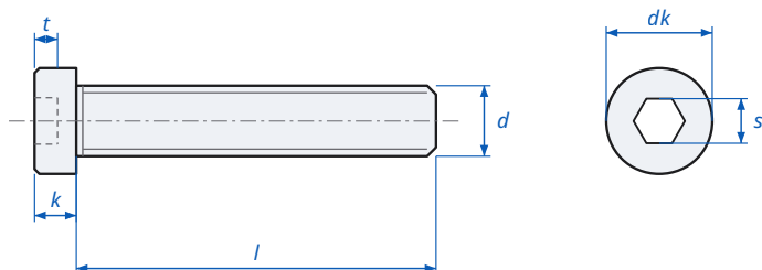
Low Head Socket Cap Screw DIN 7984 - dimensions
