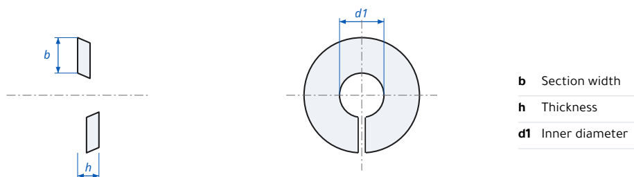
Spring Lock Washer for Socket Cap Screws DIN 7980 - dimensions
