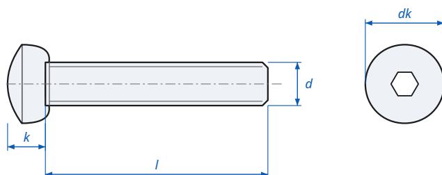
Hex Socket Button Head Screw DIN 7380 / ISO 7380-1 - dimensions
